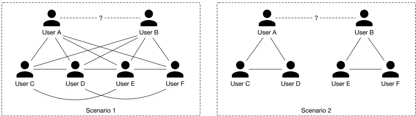
Figure 11.5: Two different scenarios of one-hop neighborhoods
