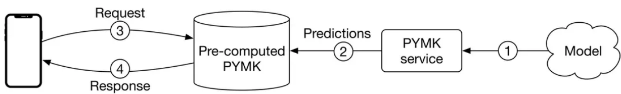
Figure 11.18: Batch prediction in PYMK
