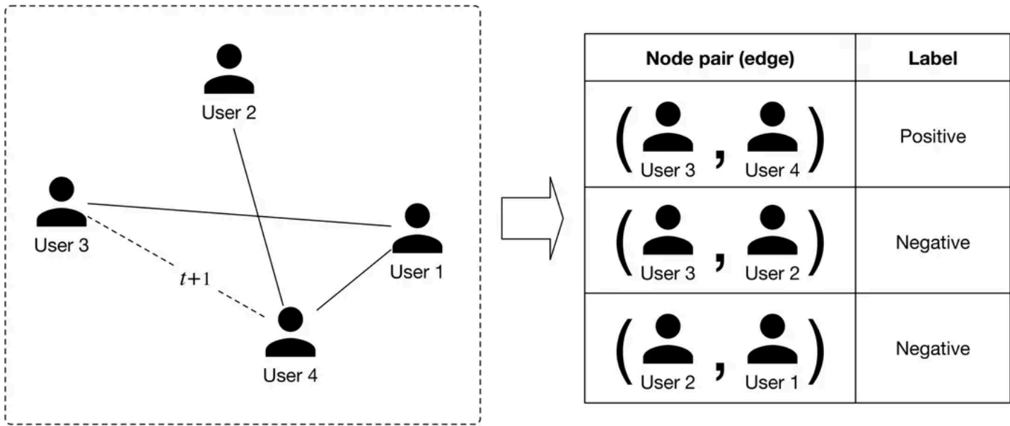
Figure 11.15: Creating positive and negative labels
