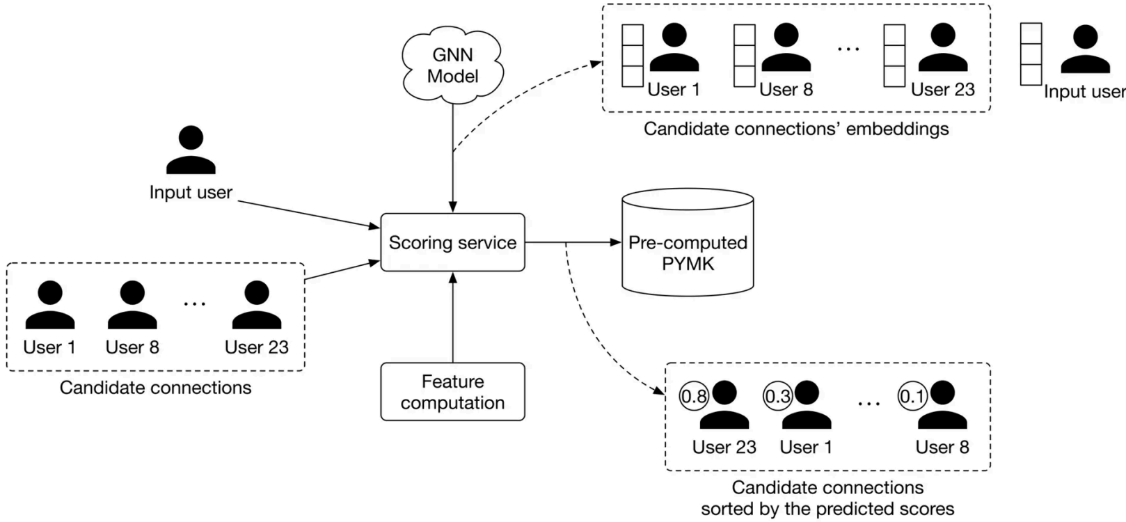
Figure 11.21: Scoring service input-output
